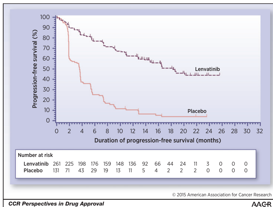
Figure 1. Kaplan-Meier plot of PFS (independent radiology review).
