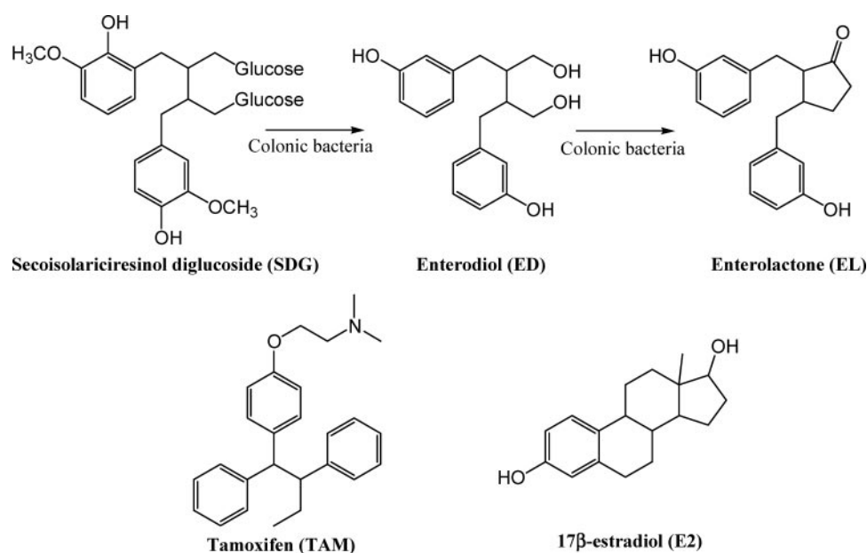
Fig. 1 Metabolism of plant lignan, SDG, to mammalian lignans, enterodiol (ED) and enterolactone (EL), and chemical structures of tamoxifen (TAM) and 17 \beta -estradiol (E2).
