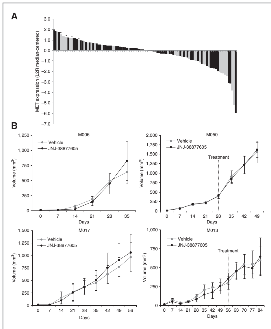
Figure 3. Lack of response to the Met inhibitor JNJ-38877605 in patient-derived xenografts of liver metastasis from colorectal carcinomas (mCRCs). A, Met expression in mCRCs. Histograms are the same as those reporting Met expression in Figure 2C. Gray histograms denote the samples that were implanted in mice for generation of treatment cohorts. Asterisks indicate the samples for which growth curves are shown in B. B, growth curves of representative patient-derived xenografts ( n = 6 for each experimental condition). Left, treatment started the day after tumor implantation; right, treatment started when the tumor had reached an established mass. Data are the means \pm SEM (error bars).
