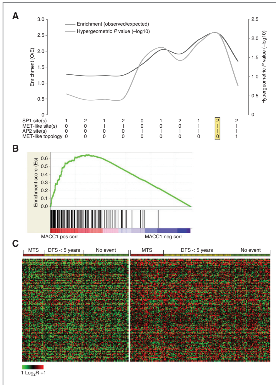
Figure 4. Identification of new putative MACC1 targets. A, enrichment statistics based on hypergeometric distribution of the Pearson correlation coefficients for the 10 genesets identified by combining Met promoter features. The SmuMA geneset, featuring the highest enrichment and hypergeometric P value, is highlighted in yellow. B, GSEA plot of the enrichment analysis for the MAput geneset in the validation dataset, GSE14333. The top portion of the plot shows the running of the enrichment score as the analysis walks down the ranked list; the lower portion of the plot shows where the members of the geneset (black lines) appear in the ranked list of genes (red-blue gradient). C, clustering of the GSE14333 dataset based on MAput expression. Samples are annotated for clinical characteristics as follows: metastatic disease at diagnosis (MTS, red samples); occurrence of metastases within a 5-year follow-up period (disease-free survival, DFS < 5 years, yellow samples); and no metastatic events during follow-up (no event, green samples).
